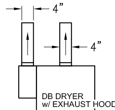
SEPERATE EXHAUST DUCT See note 1 & 3 ACCEPTABLE
