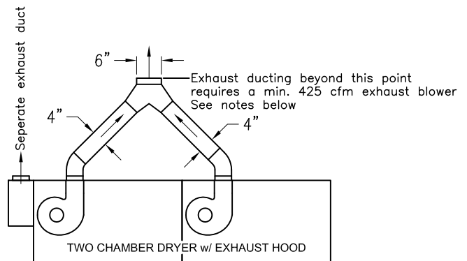
WYE JOINT DUCTING Exhaust stack blower is required See notes 1 & 2 ACCEPTABLE
