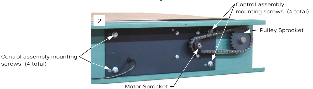
View with chain guard removed
